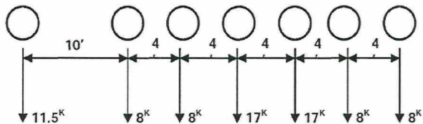
Figure 2: Single-Unit Special Hauling Vehicles, SU4-SU7
